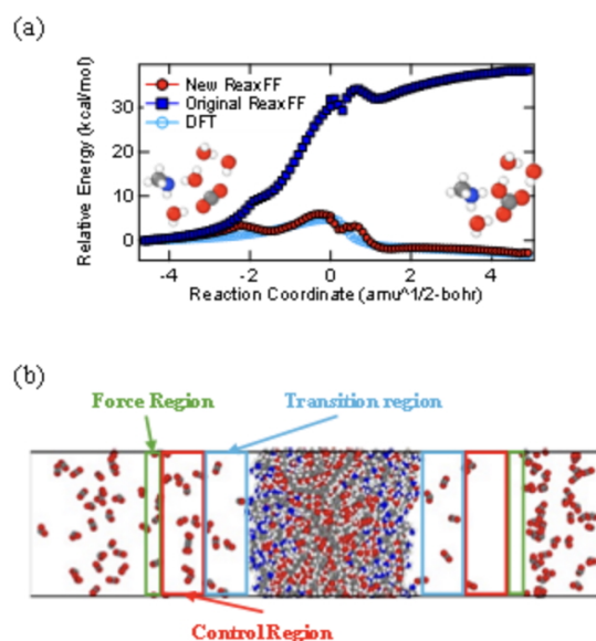
Figure 1: (a) Energy profiles along the reaction pathway calculated by newly developed ReaxFF, original ReaxFF, and DFT with 4 excess H 2 O molecules. (b) A representative snapshot of the simulation system for CGD-MD.
