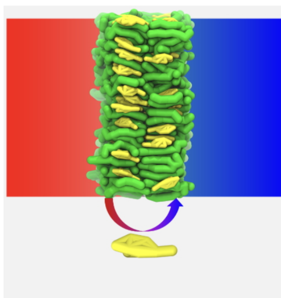
Figure 1: Representation of thermally driven cholesterol redistribution in a lipid bilayer, with cholesterol (yellow) partitioning across phospholipids (Green).
