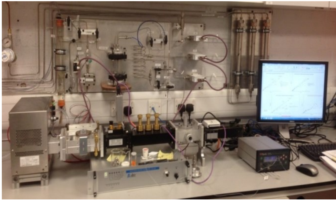
Microwave regeneration system. This system can measure the power exactly consumed by the samples, gas flow rates, CO 2 , SO 2 , NO 2 and H 2 concentrations and heating profile of the samples.
